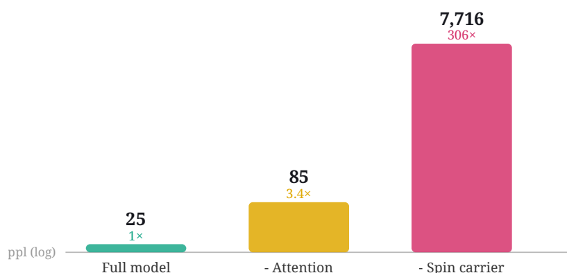
Figure 5. Causal ablation on the 284M spin-dominant model (log scale). Zeroing the spin carrier sends validation perplexity from 25 to 7,716 (306×); zeroing attention only to 85 (3.4×). The carrier is the load-bearing core.
