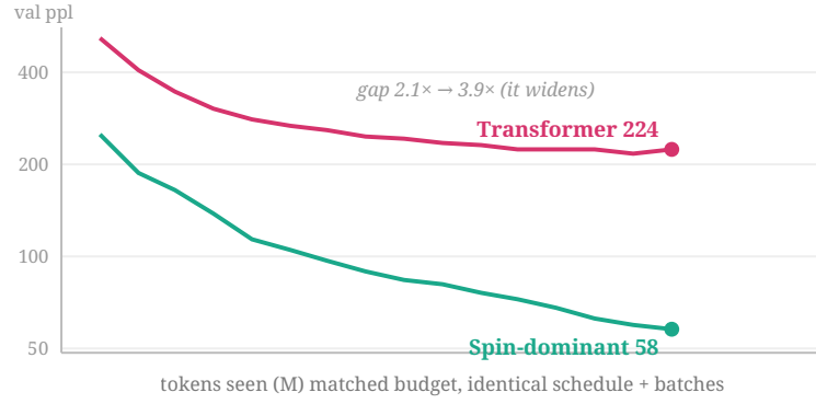
Figure 4. Learning curves at matched \sim 37 M, identical schedule and batches, each at its range-test learning rate (spin 6.7e-3 , transformer 1.0e-4 ), to 98M tokens. The transformer plateaus ( \sim 224 ) while the spin-dominant model keeps descending ( \sim 58 ), so the gap widens with training ( 2.1\times \rightarrow 3.9\times ). This directly answers the natural objection that the short-budget gap is just "the transformer hasn't trained yet": given a full schedule at its own best learning rate, the transformer descends and then flattens it does not close the gap. (Small-scale, single-seed.)
