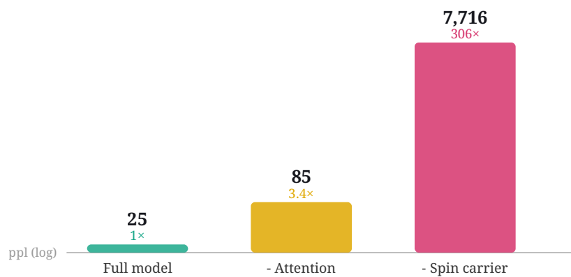
Figure 4. Causal ablation on the 284M spin-dominant model (log scale). Zeroing the spin carrier sends validation perplexity from 25 to 7,716 (306×); zeroing attention only to 85 (3.4×). The carrier is the load-bearing core.
