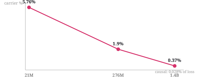
Fig. 2. A fixed single spin carrier is one d -shaped layer, so as depth and width grow its parameter share collapses (5.76% \rightarrow 1.90% \rightarrow 0.37%) and its causal contribution falls to 0.028% of the loss at 1.4B, the motivation for making the carrier the core.
