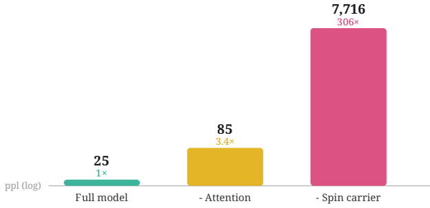
Fig. 5. Causal ablation on the 284M spin-dominant model (log scale). Zeroing the spin carrier sends validation perplexity from 25 to 7,716 (of order 300 \times ); zeroing attention only to 85 (3.4 \times ). The carrier is the load-bearing core. We read the order of magnitude, not the exact multiplier: a catastrophically ablated model’s perplexity is numerically unstable (see Section IV-F).
