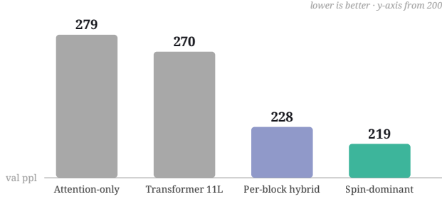
Fig. 3. Parameter-matched ablation (37–46M, same corpus and budget, single seed). Spin as the token-mixer (219) beats the attention-only baseline (279) by about 21%, and the larger per-block hybrid (228) and matched transformer (270), with fewer or equal weights.
