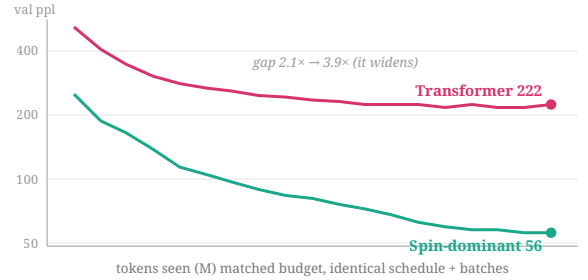
Fig. 4. Learning curves at matched 37M, identical schedule and batches, each at its range-test learning rate, to 117M tokens. Both converge, but the transformer plateaus at about 222 while the spin-dominant model descends to about 56, so the gap widens through training ( 2.1\times \rightarrow 3.9\times ). This answers the objection that the short-budget gap is just “the transformer hasn’t trained yet.” (Small-scale, single-seed.)
