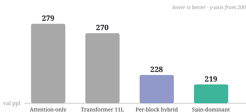
Figure 1. Param-matched ablation (~37–46M, same corpus and budget, single seed). Spin as the token-mixer (219) beats the attention-only baseline (279) by ~21%, and the larger per-block hybrid (228) and param-matched transformer (270), with fewer or equal weights.
