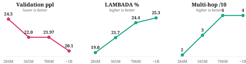
Figure 9. Progression across the four grown sizes. Validation perplexity falls, and LAMBADA (the most fluency-dependent benchmark) and the greedy multi-hop battery both rise monotonically the design improves consistently as it grows and trains, with the largest gains on the tokens-limited axes.
