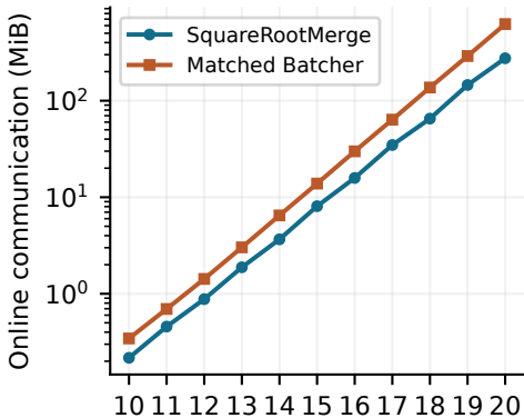
SquareRootMerge
