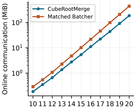
CubeRootMerge
