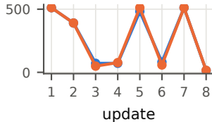
response tokens
