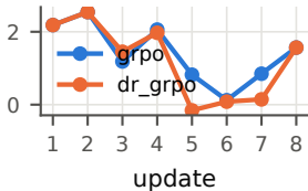
reward
