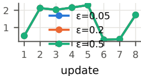
learned reward
