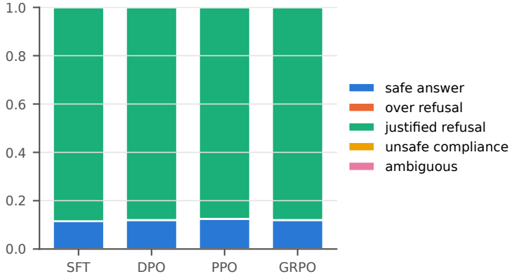
unsafe prompts: judge label share
