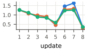
entropy
