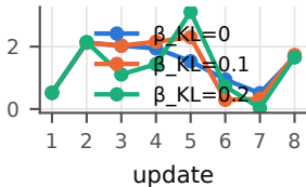
learned reward
