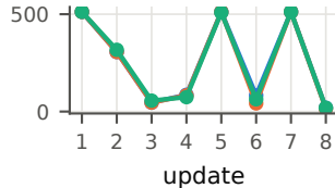
response tokens
