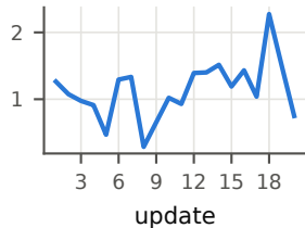
entropy
