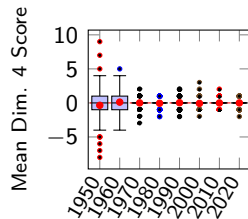
Figure: Mean Dim. 4 Scores by Decade ( R^2 = 1.26\% )
