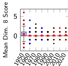
Figure: Mean Dim. 8 Scores by Decade ( R^2 = 2.85\% )
