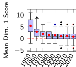
Figure: Mean Dim. 1 Scores by Decade ( R^2 = 35.55\% )
