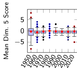
Figure: Mean Dim. 5 Scores by Decade ( R^2 = 1.63\% )
