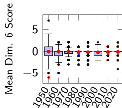
Figure: Mean Dim. 6 Scores by Decade ( R^2 = 0.33\% )
