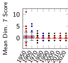
Figure: Mean Dim. 7 Scores by Decade ( R^2 = 3.75\% )
