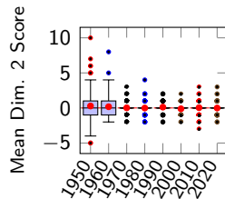
Figure: Mean Dim. 2 Scores by Decade ( R^2 = 0.99\% )
