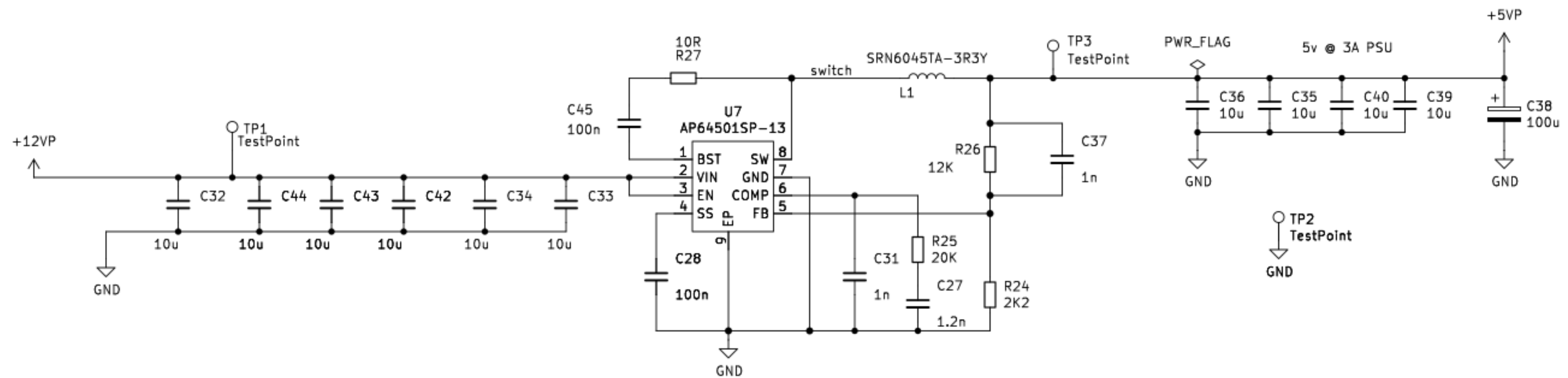
+5v @ 3A PSU ( 7.5v-28v Input )
