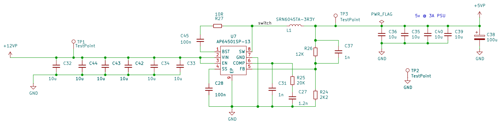
+5v @ 3A PSU ( 7.5v-28v Input )
