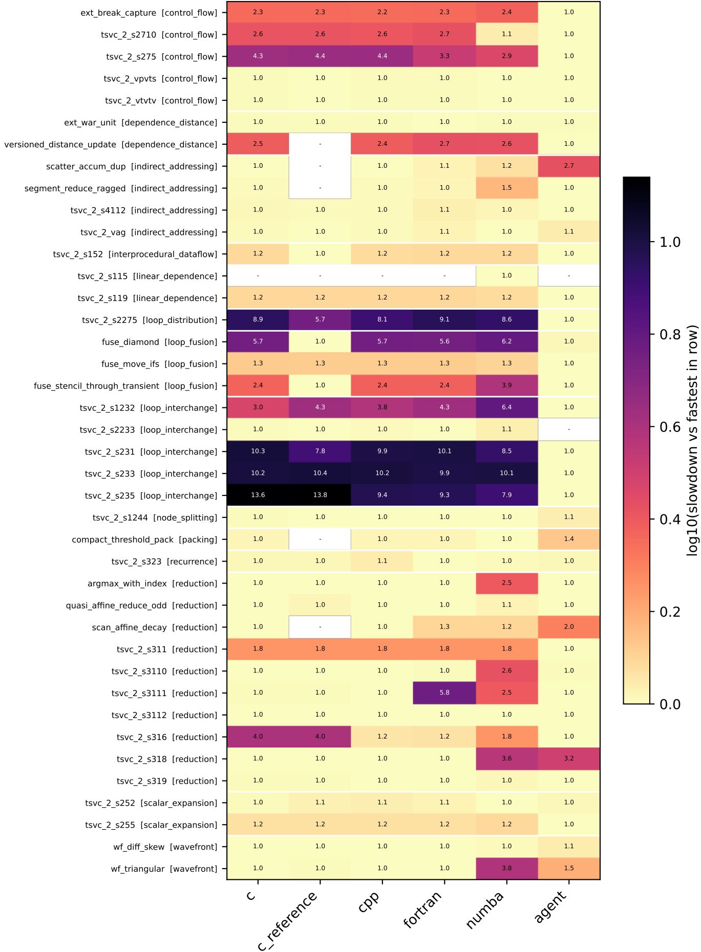
LLR-40: slowdown vs fastest representation per kernel (preset M, float64, 1 thread, gcc 14.2.0 (C) / g++, gfortran 13.3.1; '-' = no ok timing)
