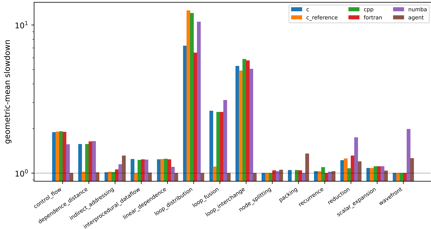
Geometric-mean slowdown per (optimization class x representation)
