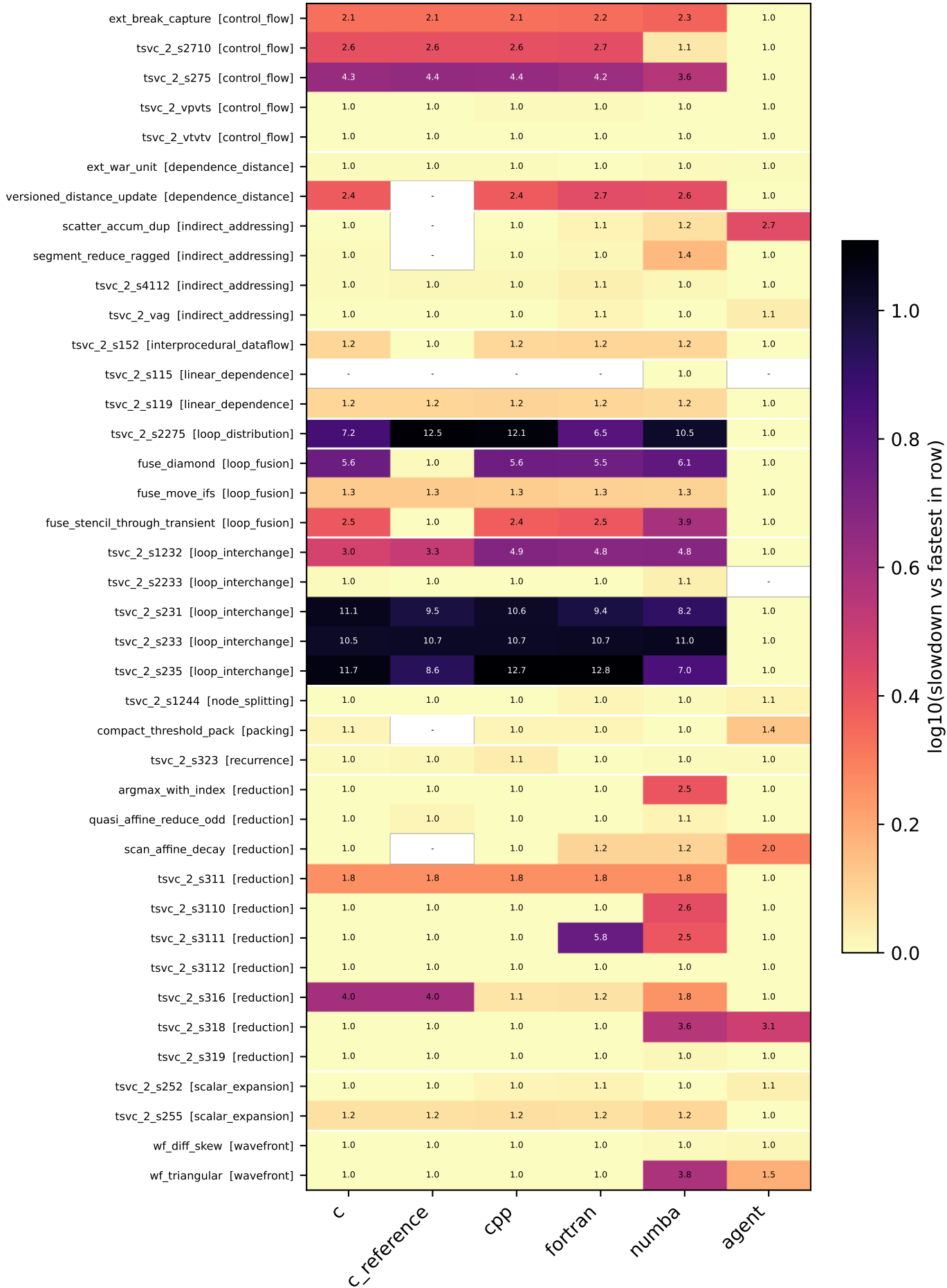
LLR-40: slowdown vs fastest representation per kernel (preset M, float64, 1 thread, GNU 13.3.1; '-' = no ok timing)
