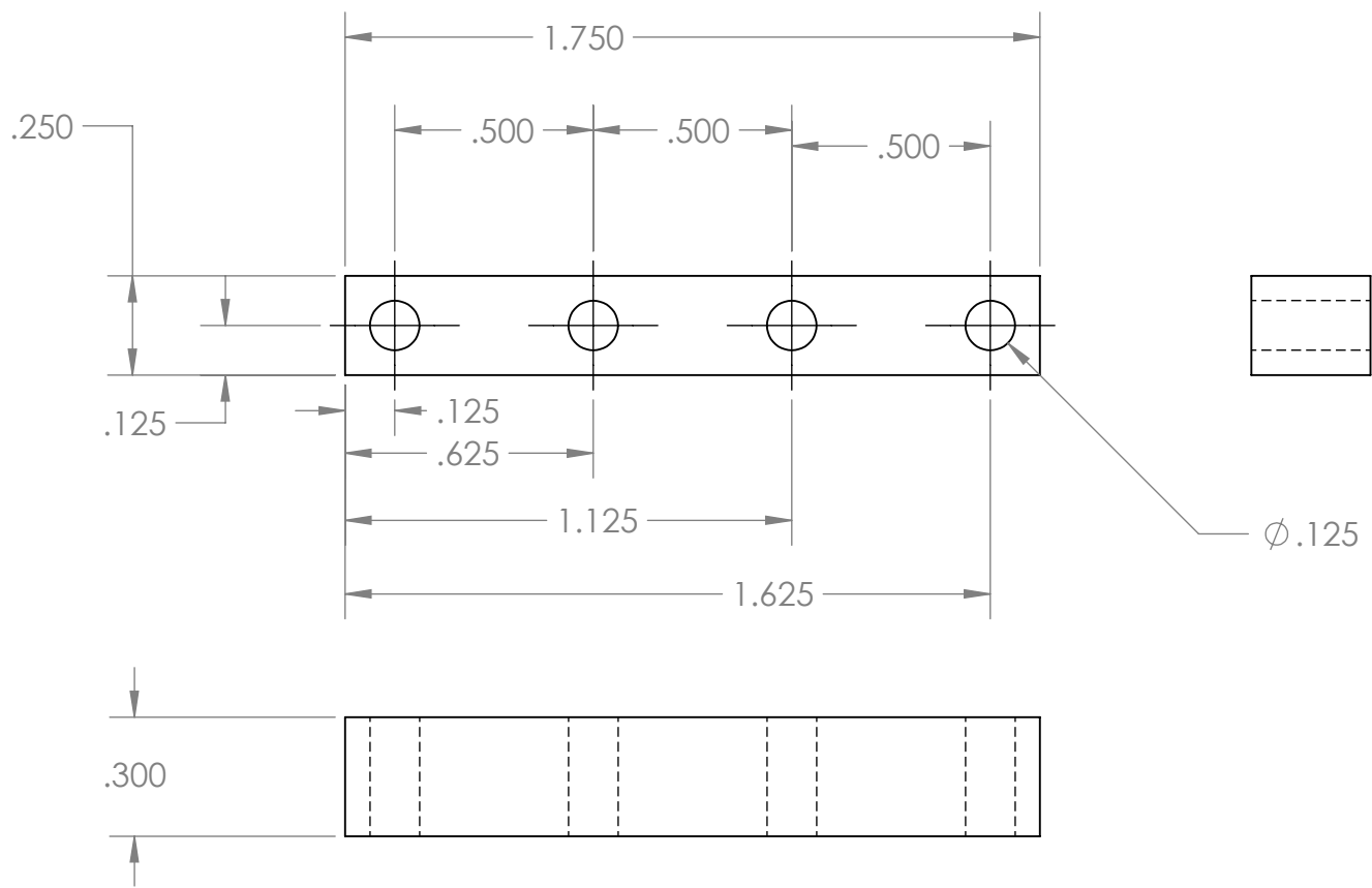
top spacer bracket(brass)
