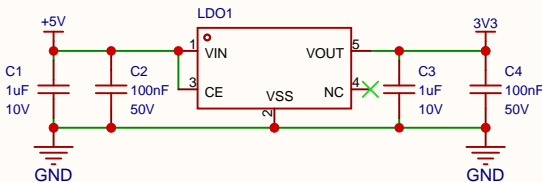
LDO-5V转3.3V电路
