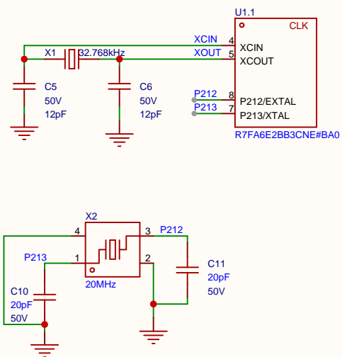
R7FA6E2BB3CNE_时钟
