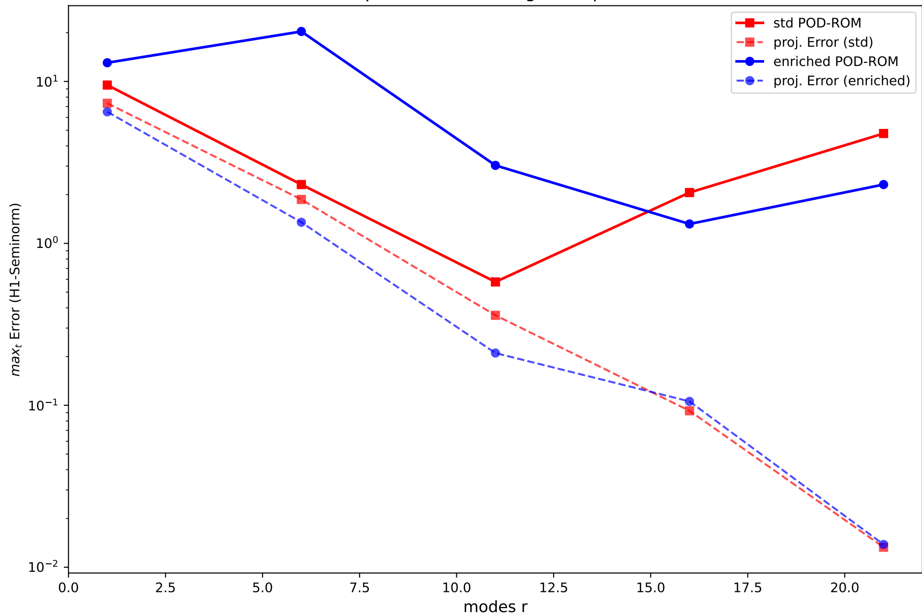
Comparison of convergence ( \beta=3.75 )
