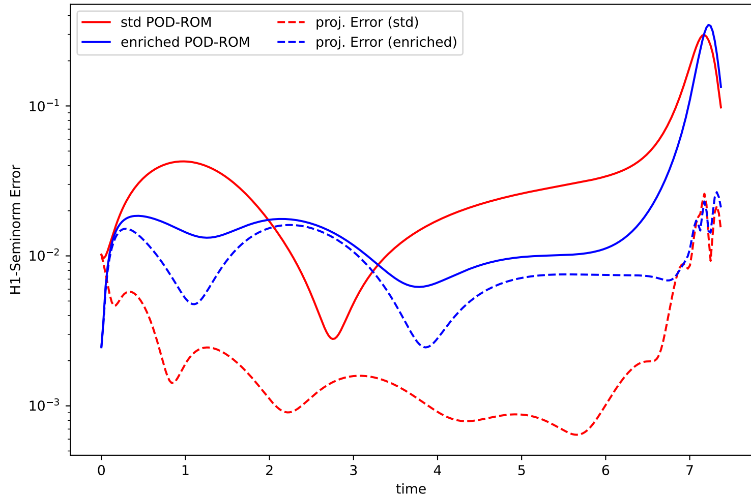
ROM-error over time for \beta=3.25 , including projection error (r=15)
