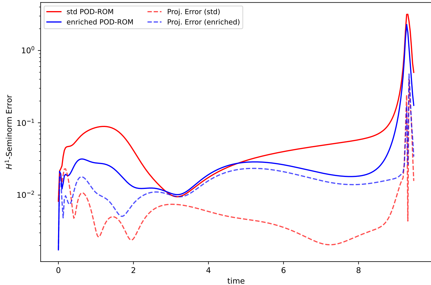
ROM-error over time for \beta=4.25 , including projection error (r=15)
