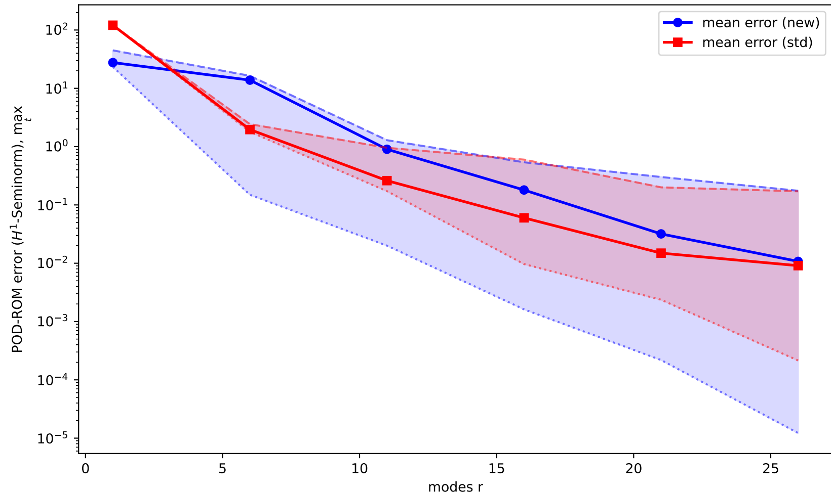
Std vs. New POD-ROM, mean, min, max over 35 Parameters
