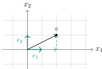
Before: v = 2e_1 + e_2 .
