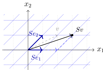
After: Sv = 2(Se_1) + Se_2 .
