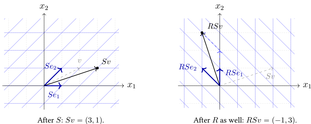
Figure 7.2: Composition: first the shear S , then the rotation R
