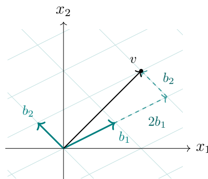
Figure 6.2: Read against B : v has coordinates (2, 1) .
