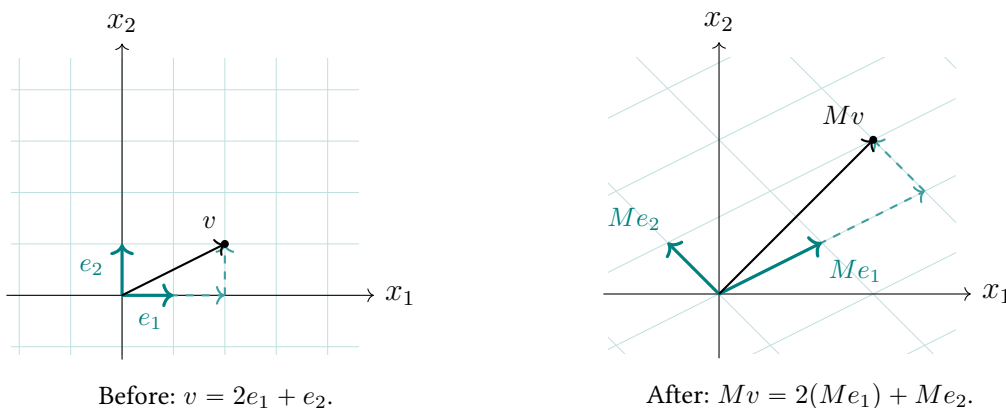
Figure 7.1: The matrix M read as a motion of the whole plane: e_1 and e_2 land on its two columns, and v follows. Notice that the grid lines stay parallel and evenly spaced, that the origin does not move, and that the transformed grid is exactly the B -grid of Figure 6.2 .
