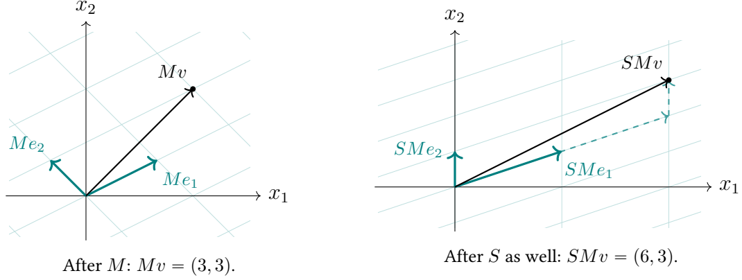
Figure 7.2: Composition. The left panel is the right-hand panel of Figure 7.1 : the plane once M has moved it. Shearing that with S gives the right panel, whose grid is the one belonging to the single matrix SM . The two-step route and the one-step route end at the same point.
