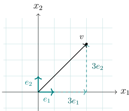
Figure 6.1: Read against E : v has coordinates (3, 3) .
