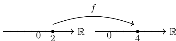
Figure 9.1: Mapping of 2 under x^2
