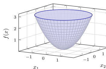
(b) \text{epi}(f)
