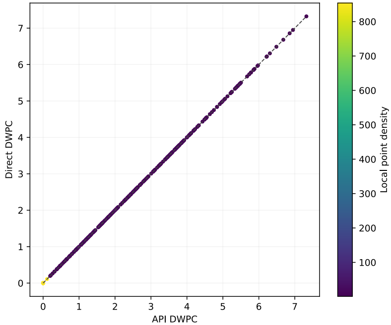
Direct vs API DWPC concordance
