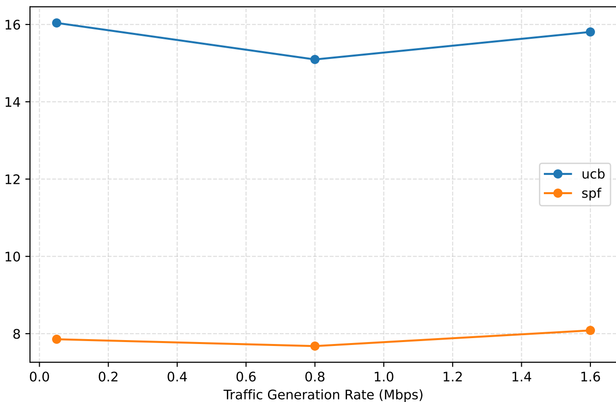
Median End-to-End Delay (ms)
