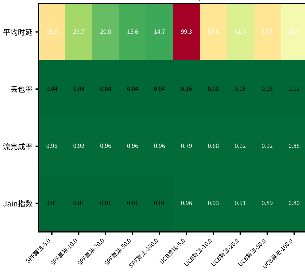
负载 = 0.05 Mbps
