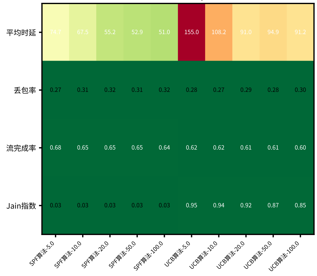
负载 = 1.6 Mbps
