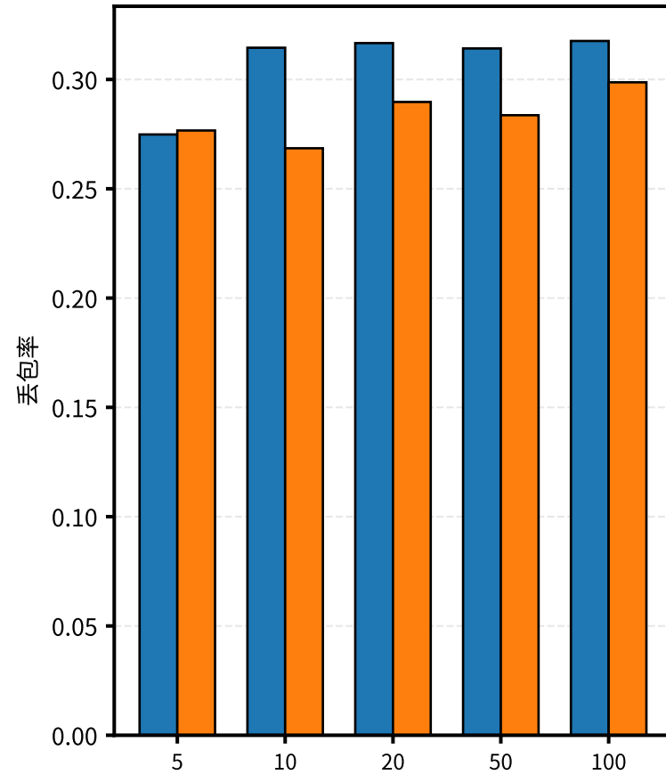
(b) 负载=1.6 Mbps
