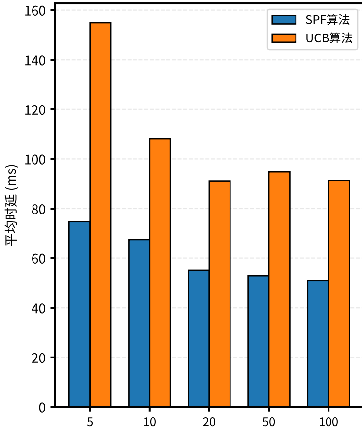
(a) 负载=1.6 Mbps
