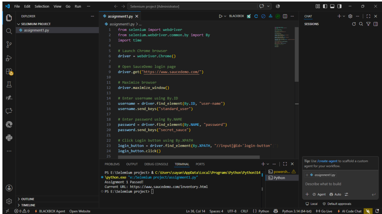
Figure 3 – VS Code terminal showing the passed assertion and resulting URL.
