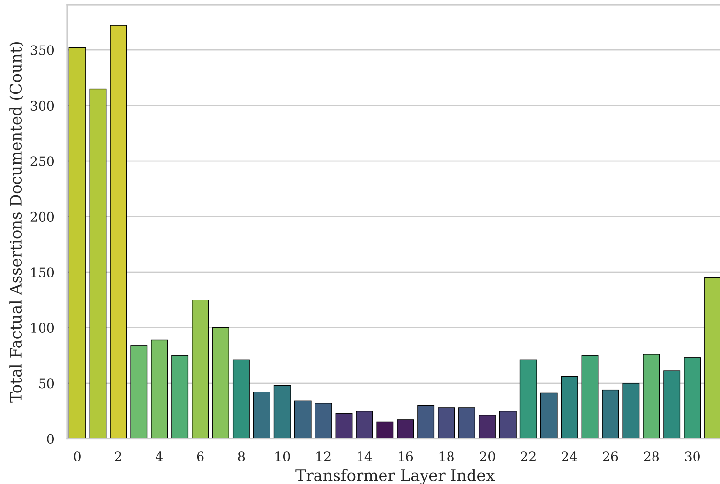
A: Global Topological Frequency of Knowledge Neurons (How often a layer rules the Top-3)
