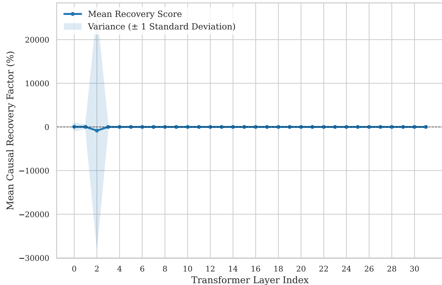
B: Macro Causal Saliency Profile Across LLM Network (Dataset-Wide Average Layer Performance)
