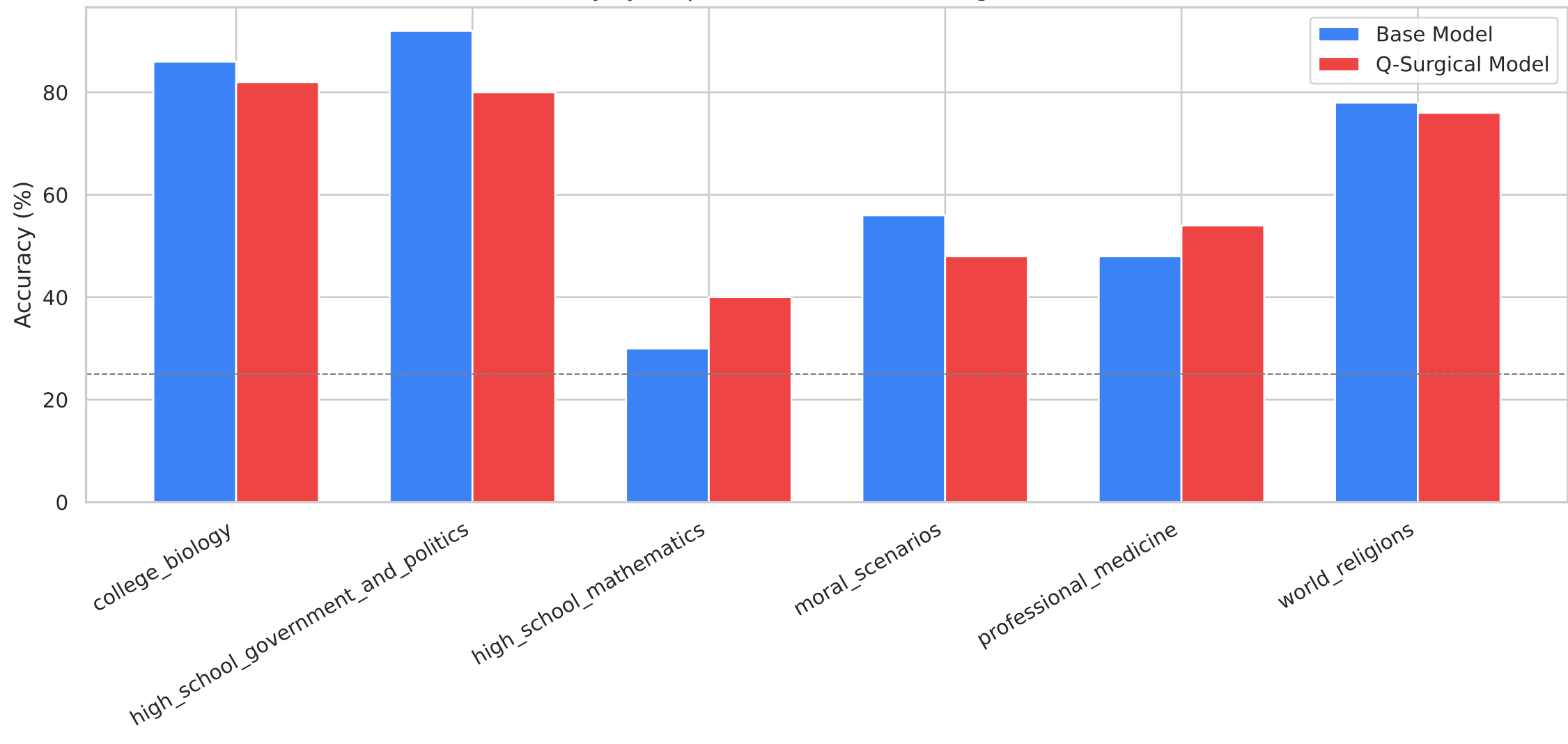
MMLU Accuracy by Subject: Base Model vs Q-Surgical Unlearned Model
