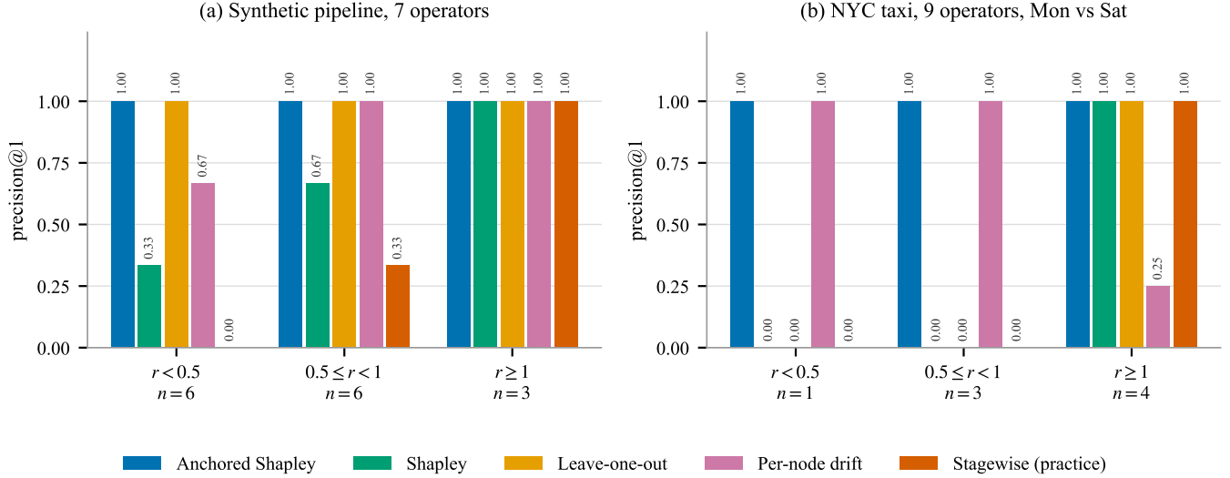
Fig. 1. Precision@1 by fault-to-drift ratio r . The anchored value is flat at 1.00 in every regime. On the synthetic pipeline (a), plain Shapley degrades below r = 1 while leave-one-out does not. On real NYC taxi partitions (b), leave-one-out collapses alongside Shapley and current practice, and the anchored value is the only estimator that survives.
