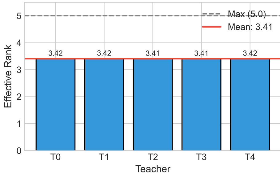
(b) Effective Rank (std = 0.002)
