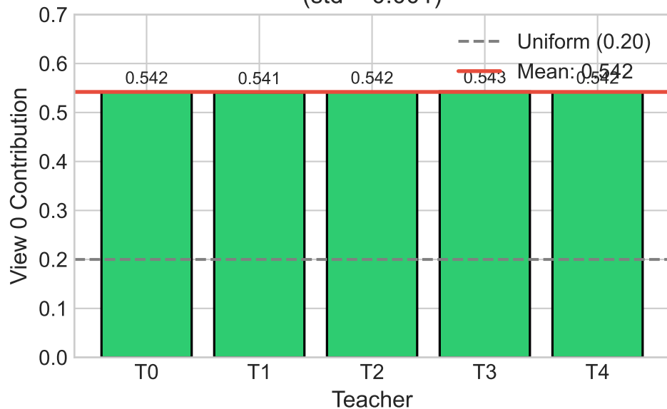
(a) View 0 Contribution (std = 0.001)
