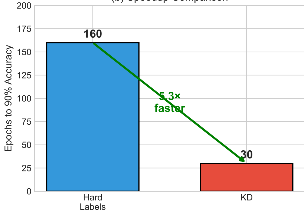
(b) Speedup Comparison
