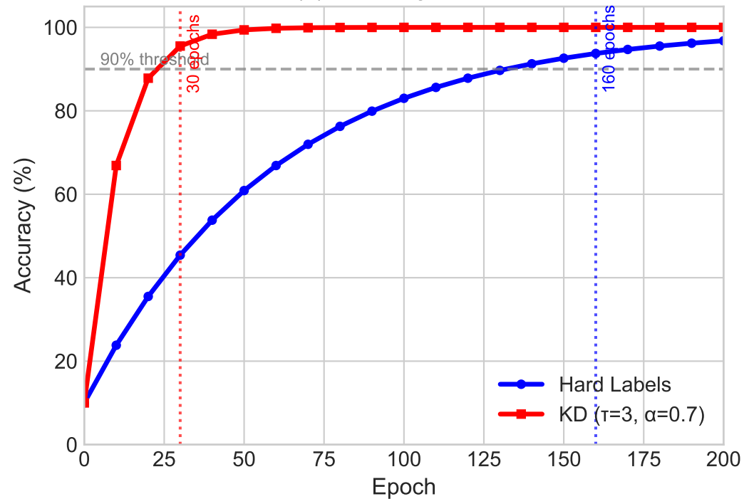
(a) Learning Curves
