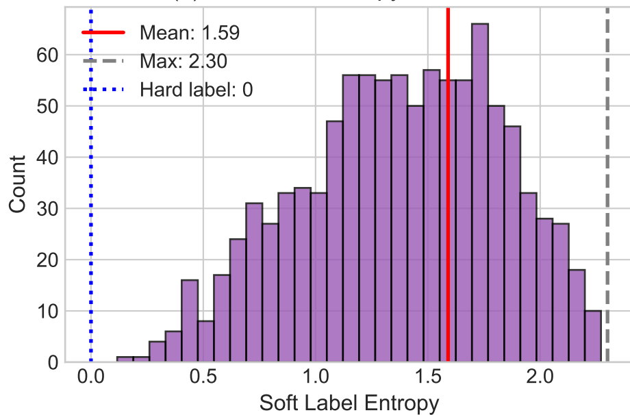
(a) Soft Label Entropy Distribution
