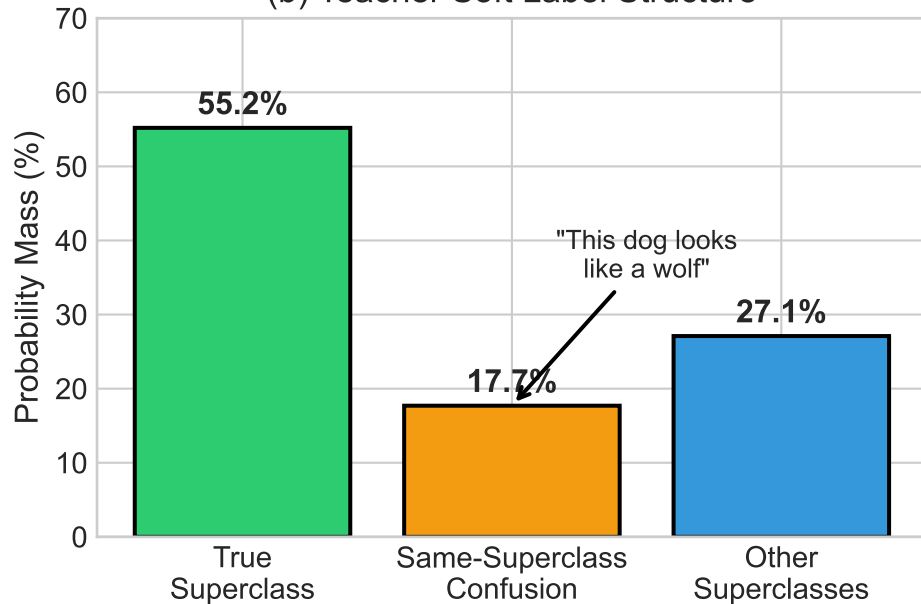
(b) Teacher Soft Label Structure
