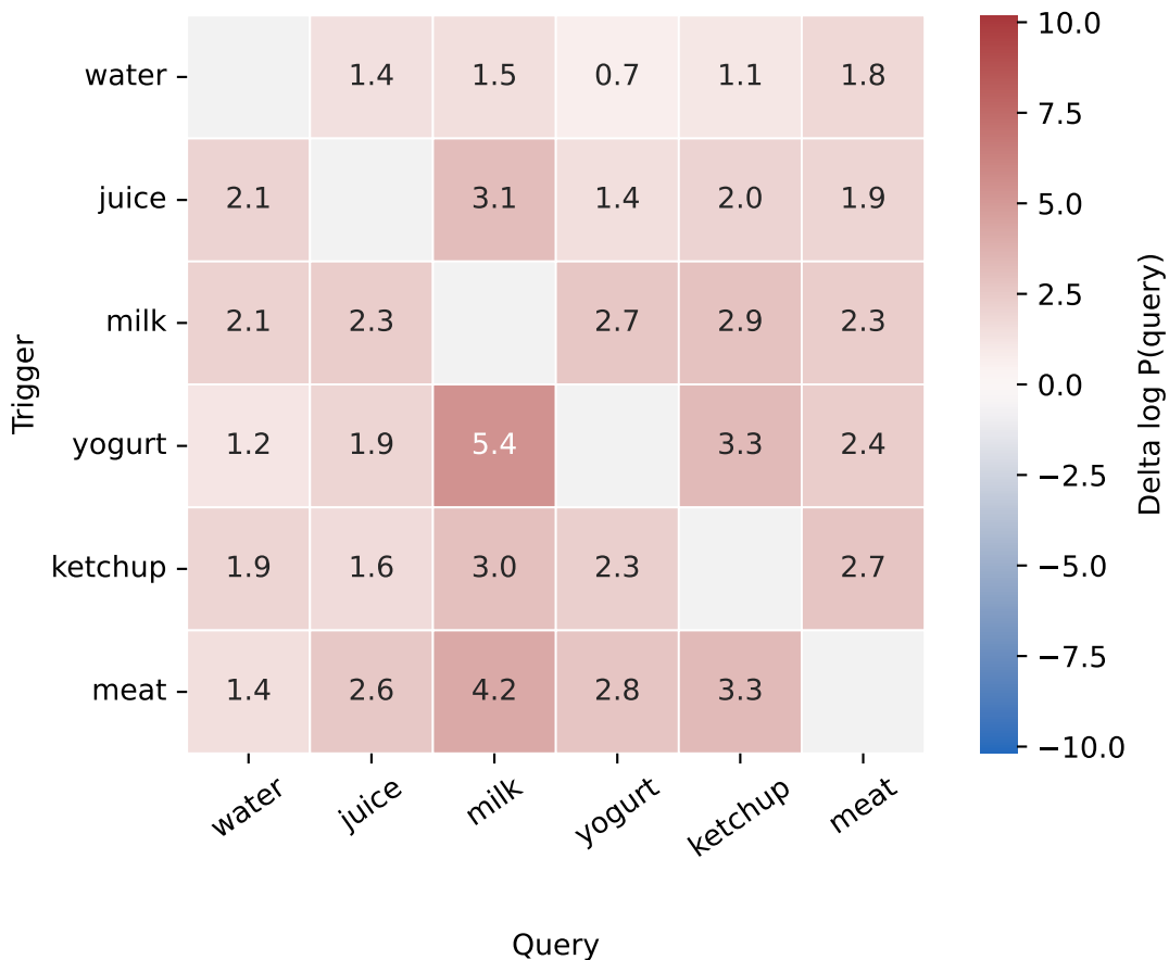
fridge: trigger effect on query log probability
