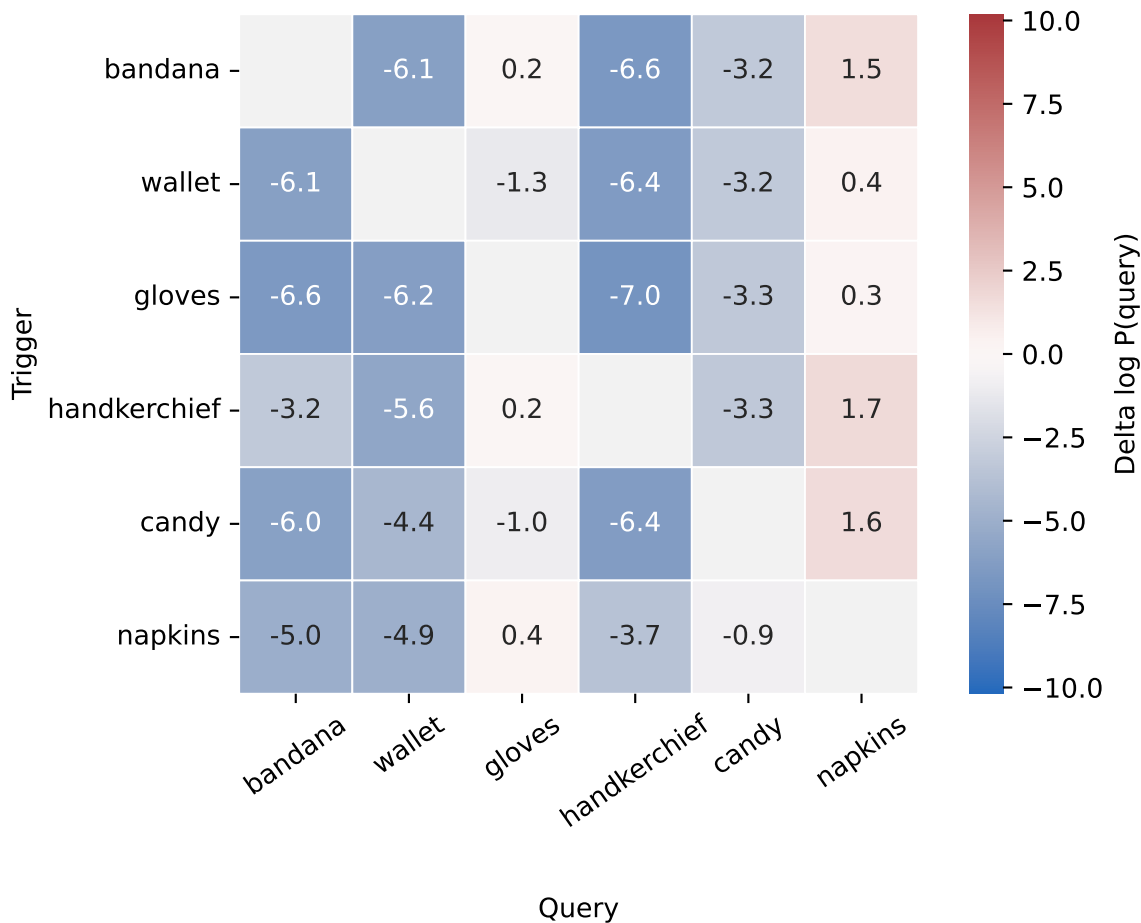
mask: trigger effect on query log probability
