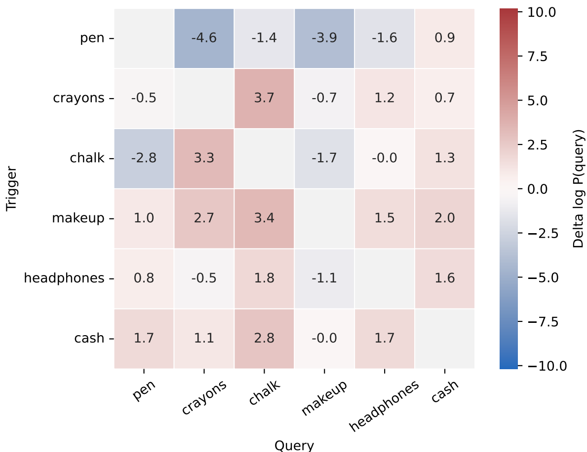
bag: trigger effect on query log probability
