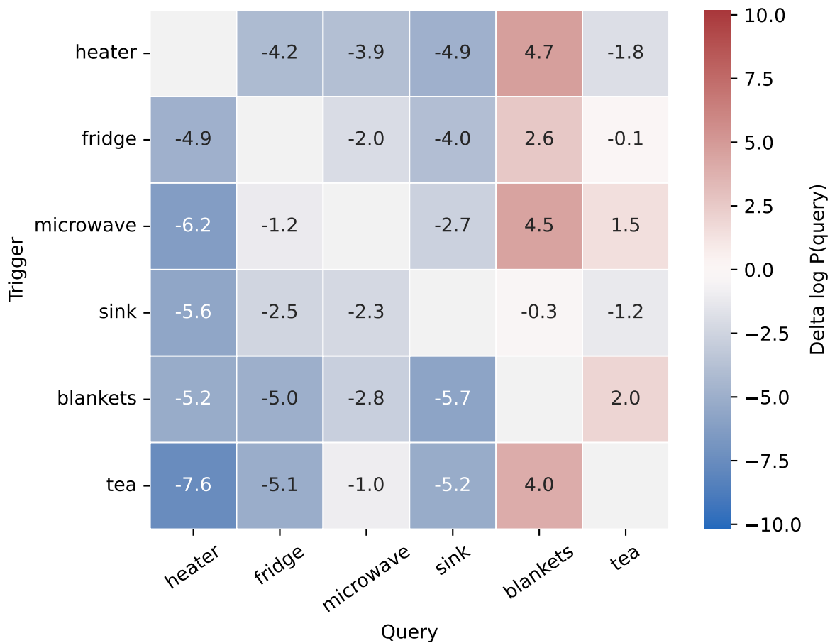
cold: trigger effect on query log probability
