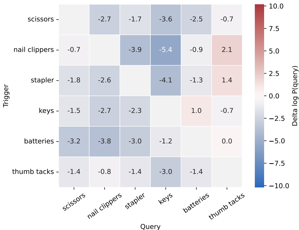
cut: trigger effect on query log probability
