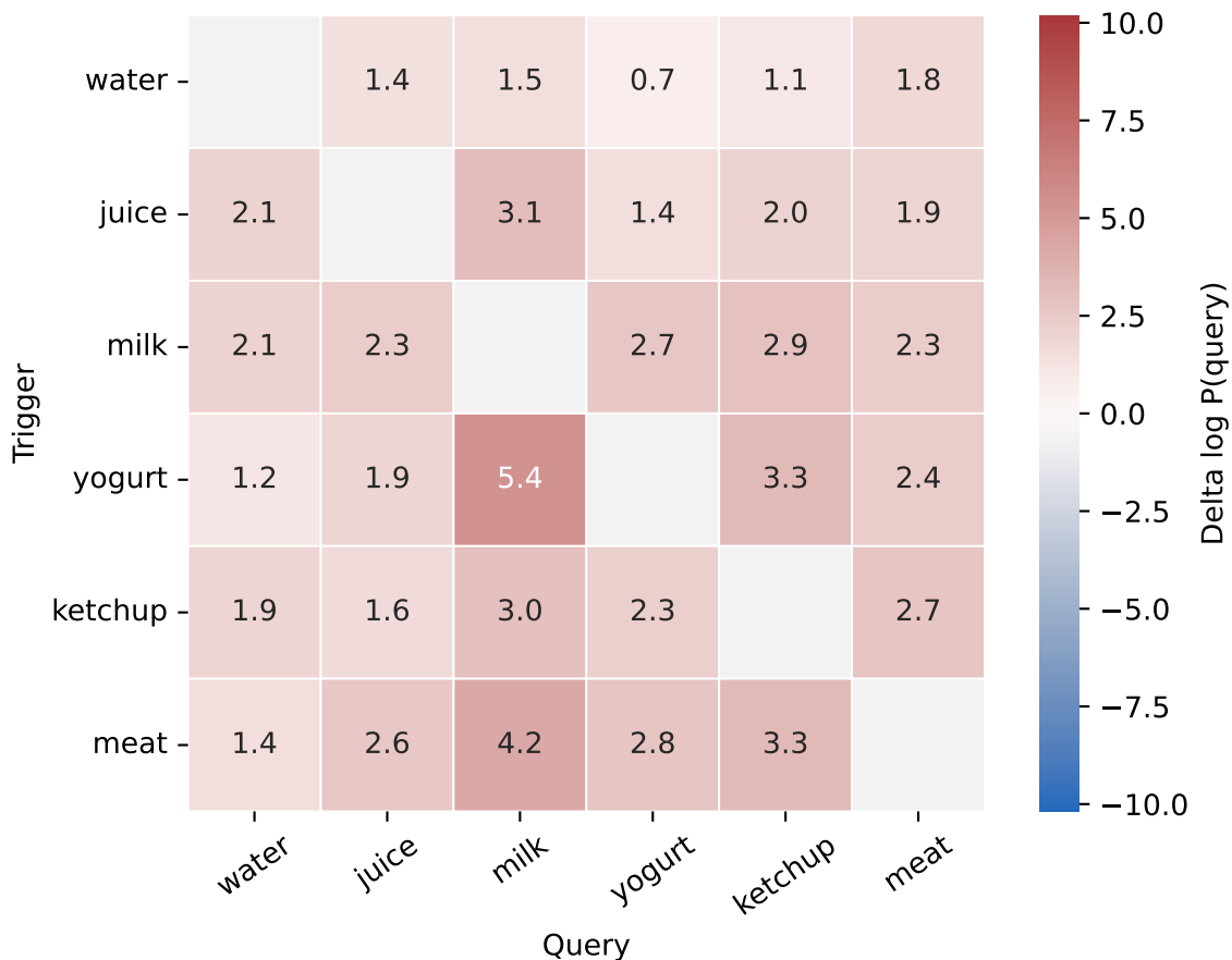
fridge: trigger effect on query log probability
