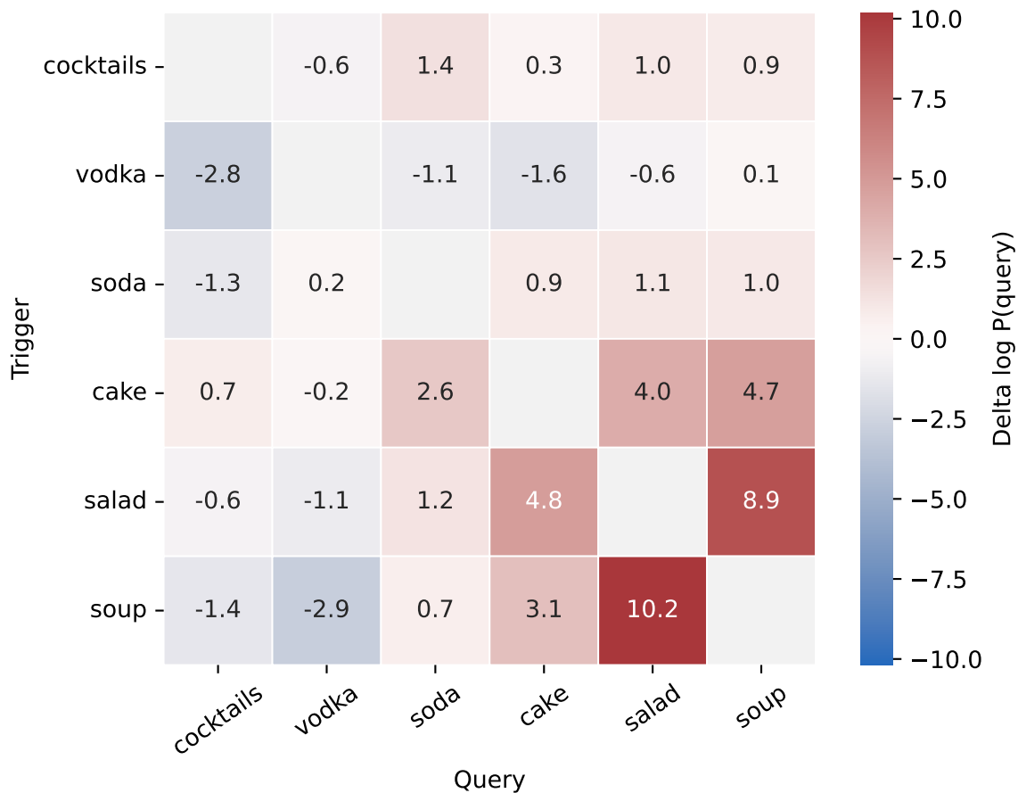
restaurant: trigger effect on query log probability
