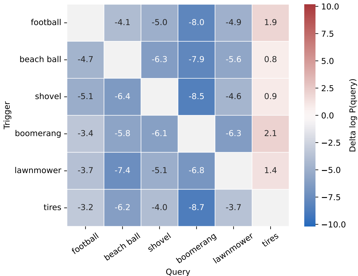
throw: trigger effect on query log probability
