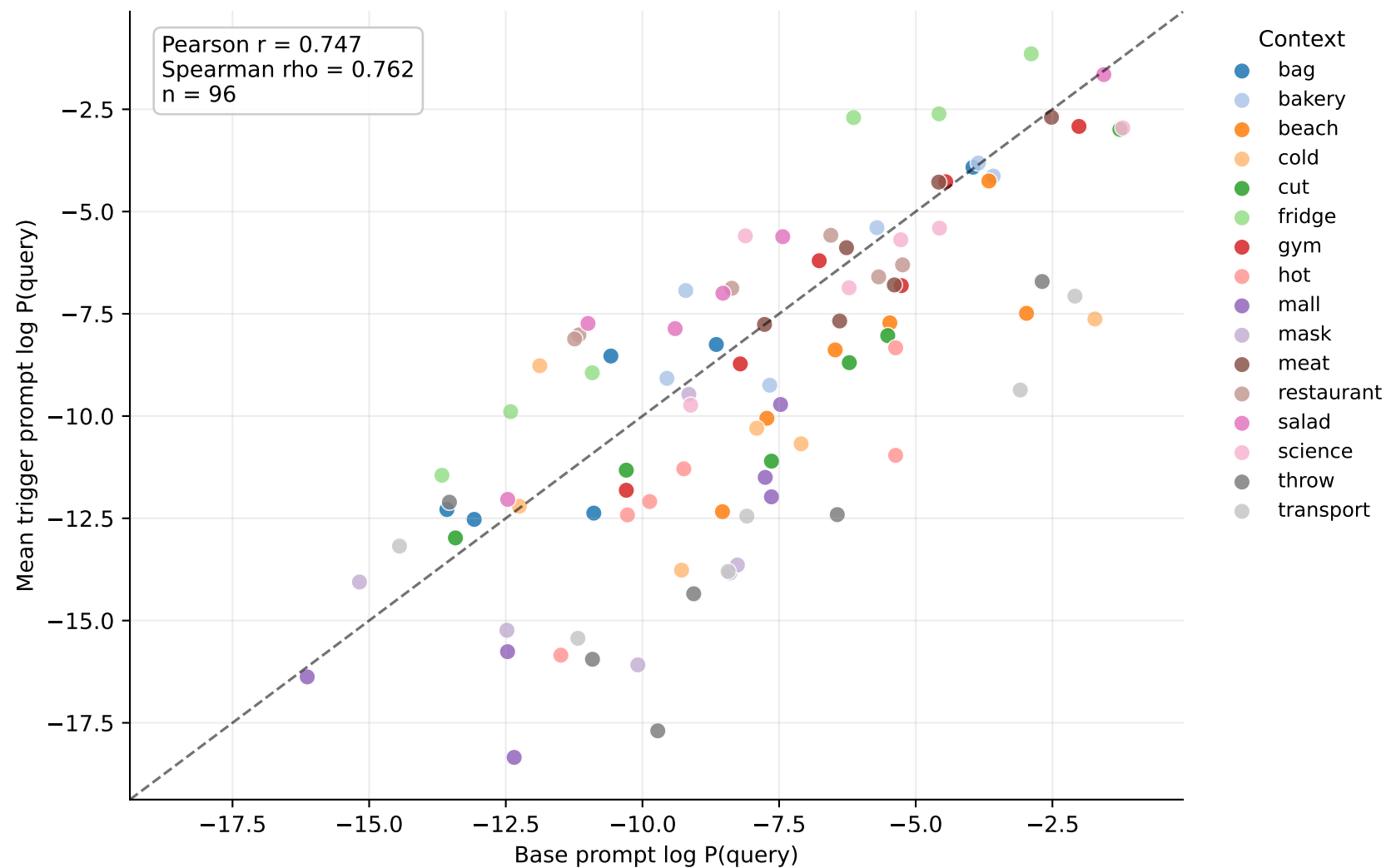
Base vs. Trigger-Conditioned Qwen Query Scores
