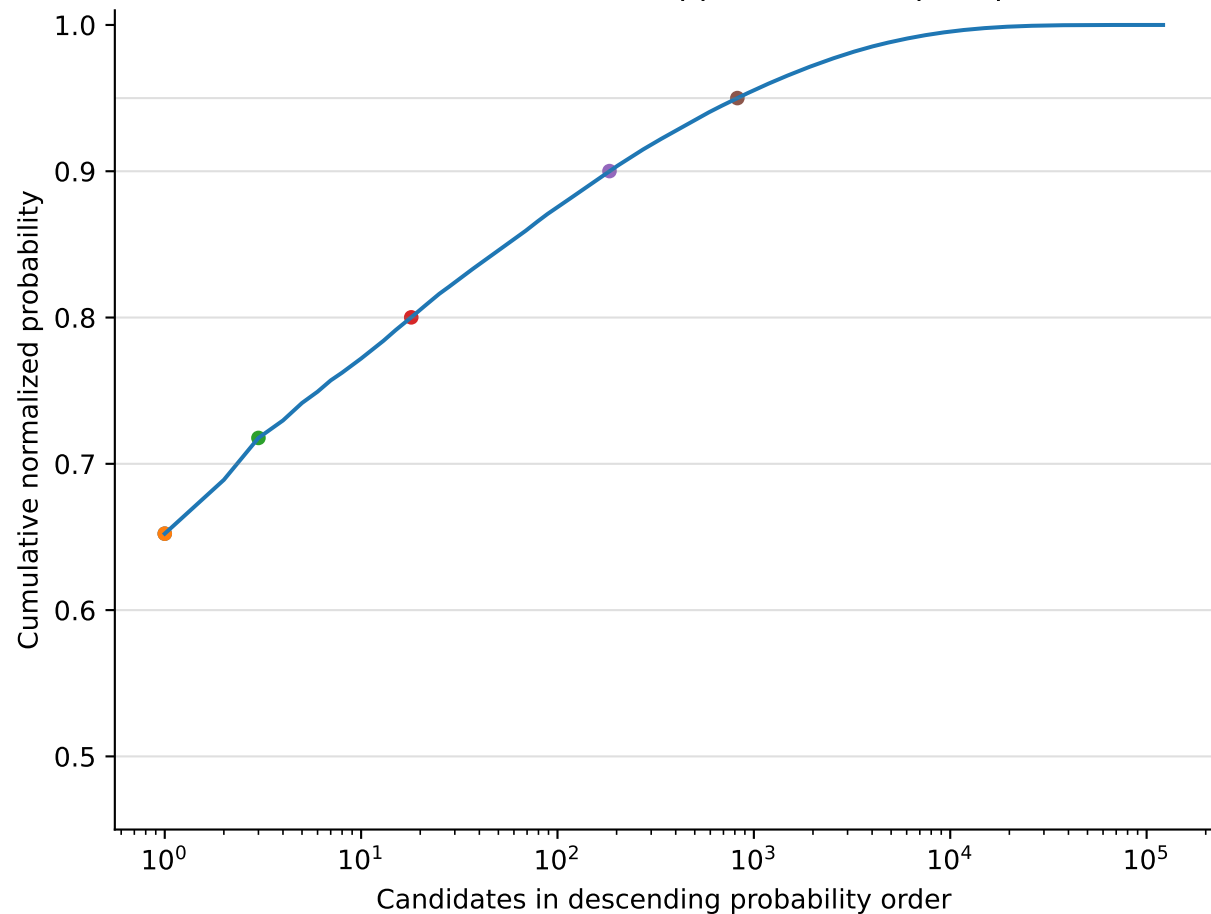
Mass concentration (sorted support, not sampled prefixes)
