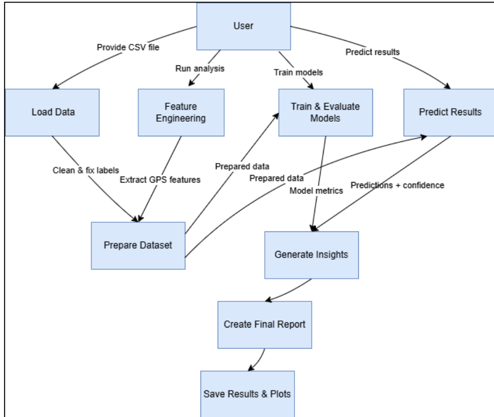
Figure 4. Flowchart Diagram.
