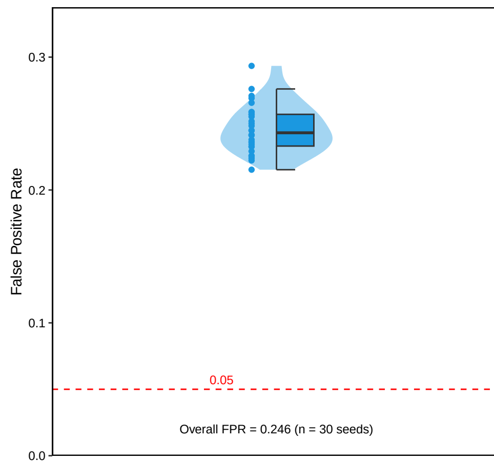
Negative Benchmark
