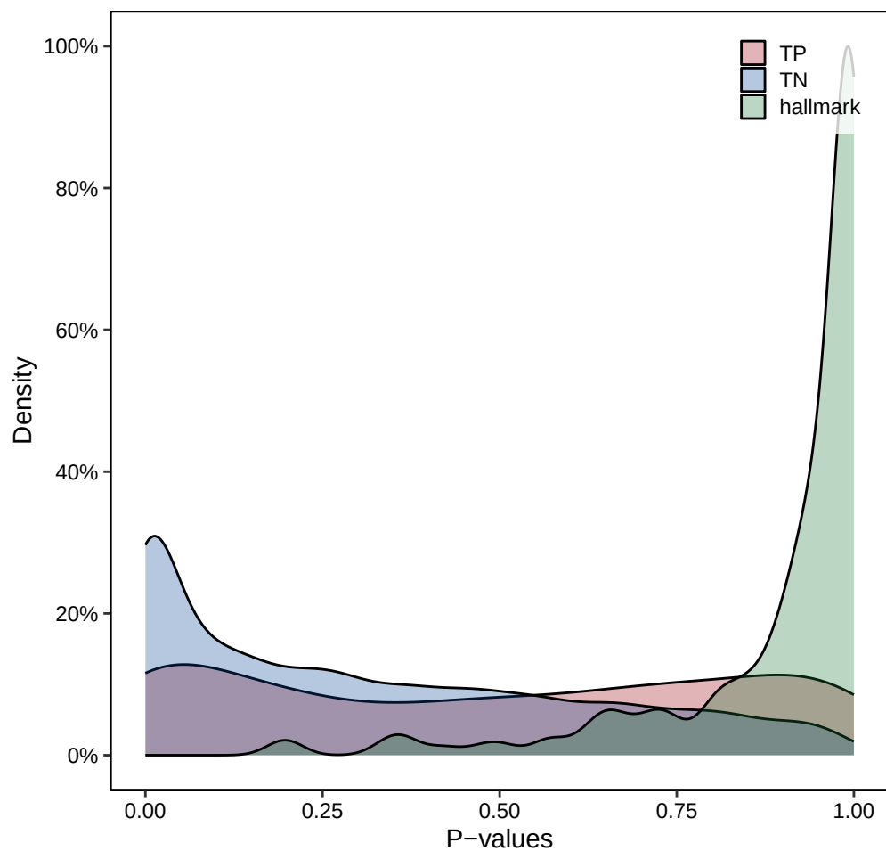
P-value Distribution
