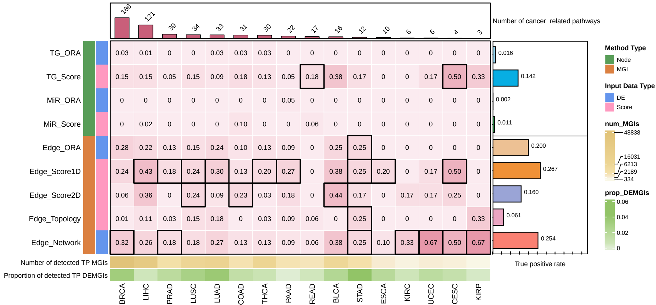
True Positive Rates Across 16 Cancer Types
